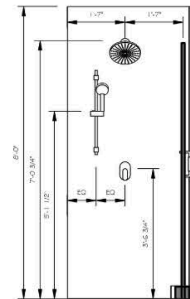
5 ENS. SHOWER WALL SCALE: 3/8" = 1'-0"
